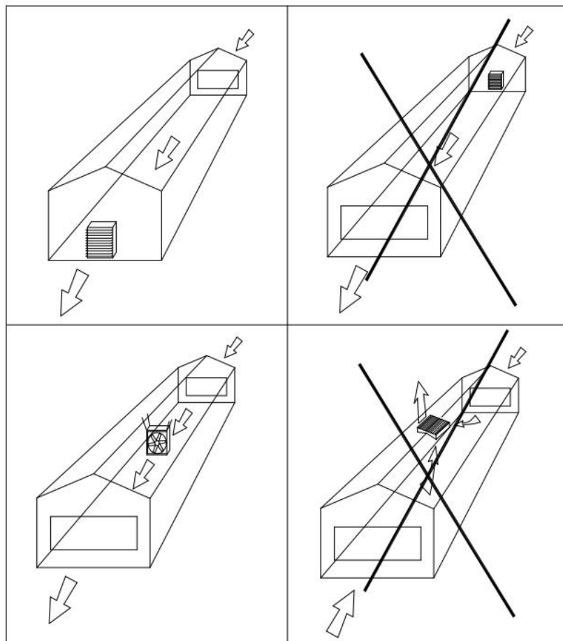
Installation diagram
