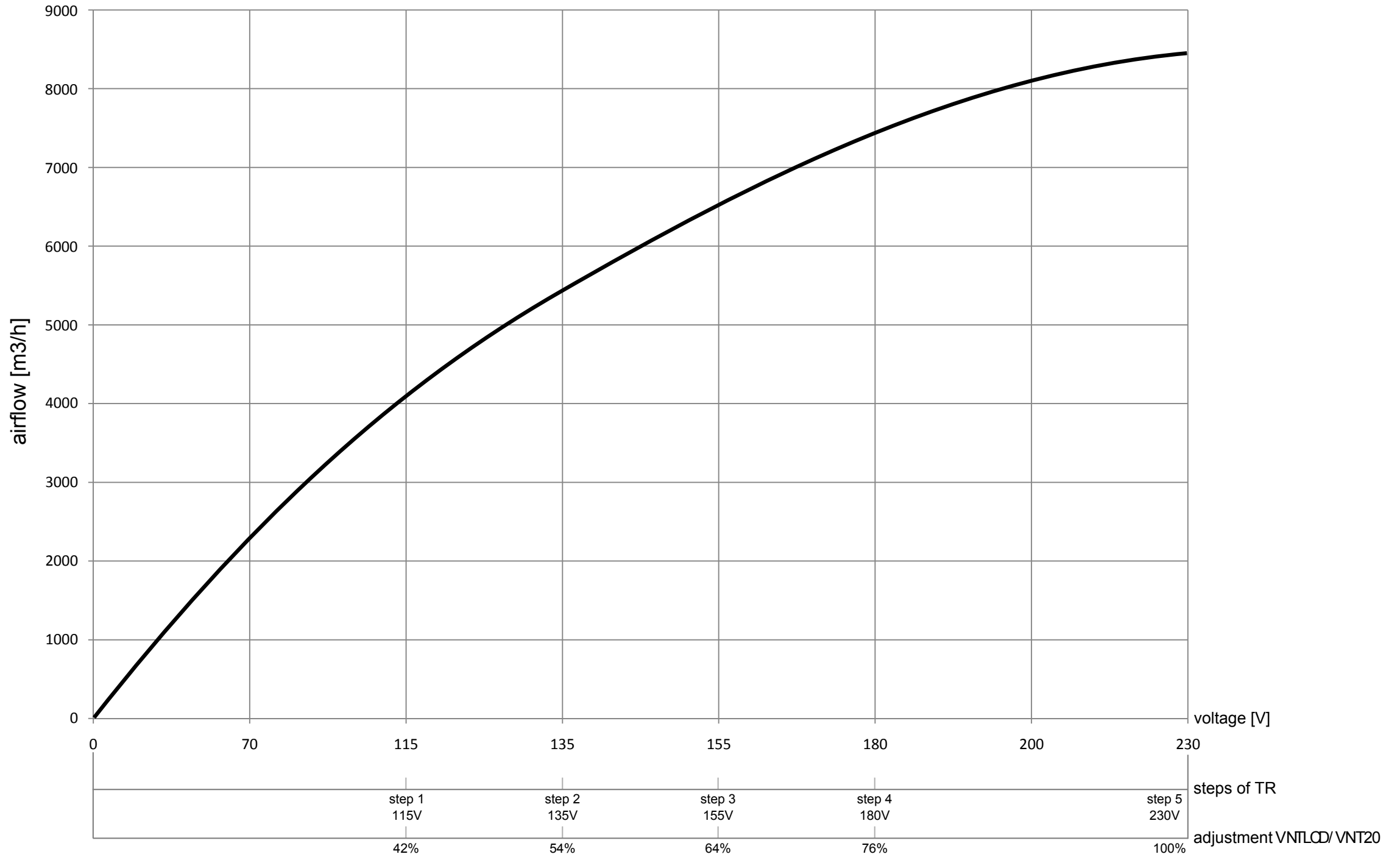
The airflow diagram of the LEO FB 95 in dependence of the TR/VNTLCD/VNT20 adjustment
