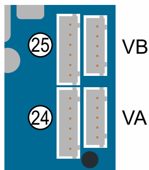
FIG. 16 (Outputs for the electronic expansion valves on the μKita electronic control board)
