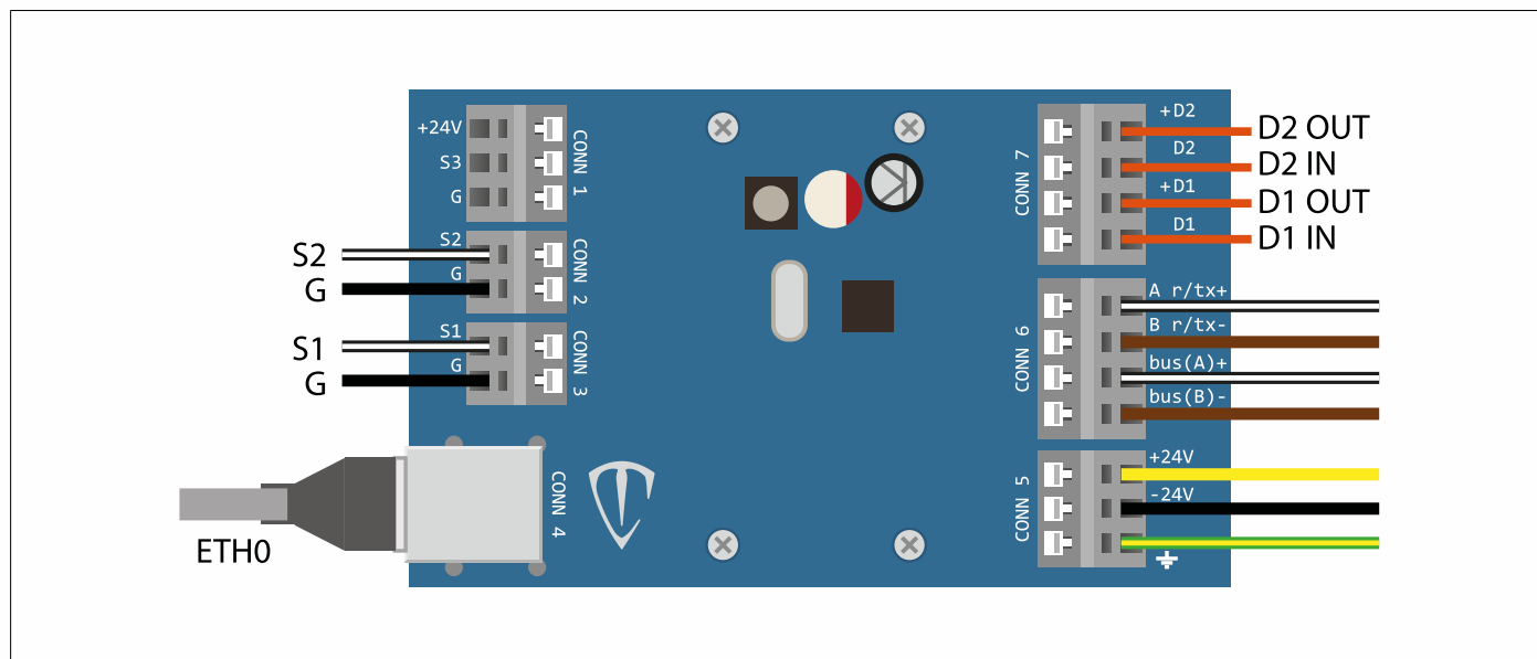
FIG. 8 SG-Probe electronic board
