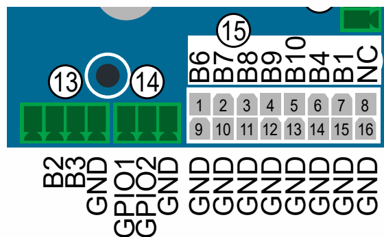
FIG. 13 (Temperature probe inputs on the µKita electronic control board, connectors 13 and 14)
