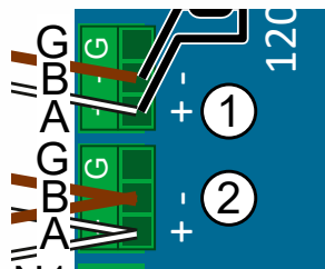
FIG. 9 (Connectors 1 and 2)
