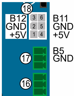
FIG. 14 (Inputs 4–20 mA on the \mu Kita electronic control board, connectors 17 and 18)
